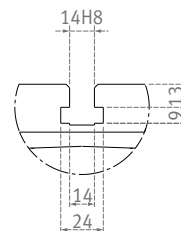
Detail B (1:2)
