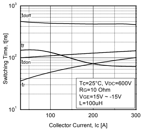
Fig 5. Typical Switching Time vs Collector Current
