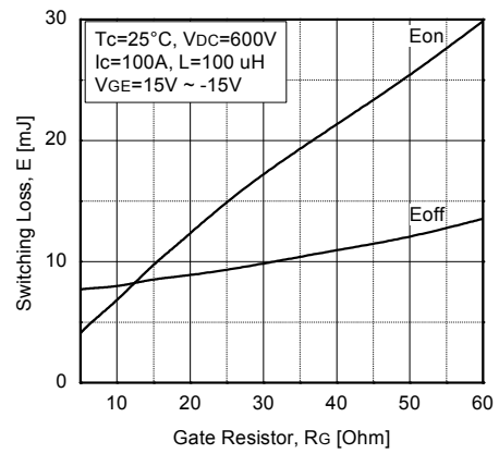
Fig 8. Typical Switching Loss vs Gate Resistor
